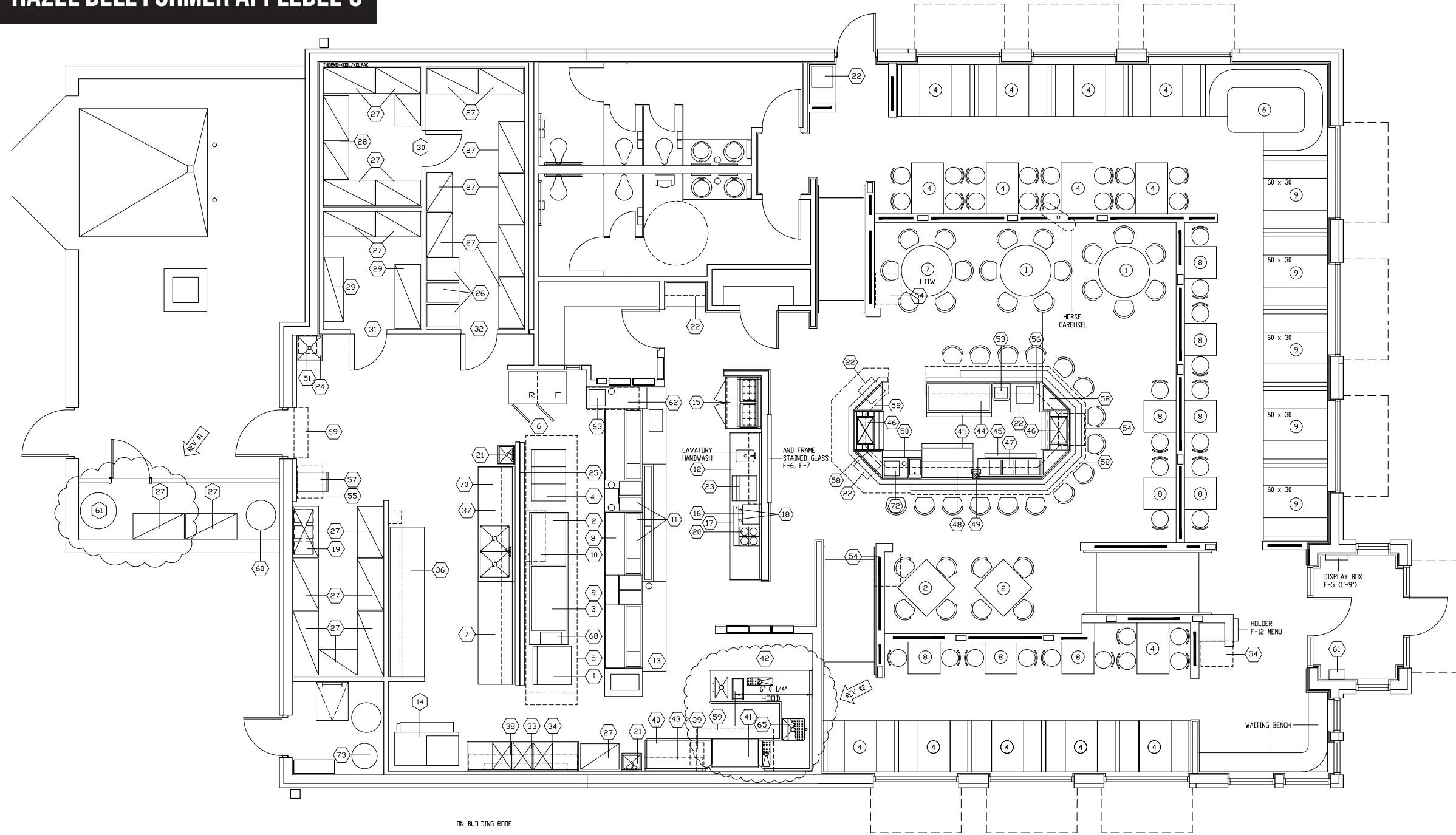
1 FURNITURE & EQUIPMENT PLAN 1/4"
